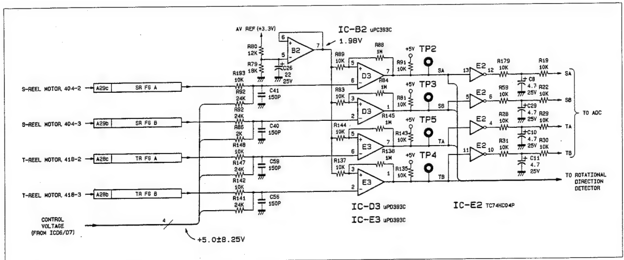
Fig. 4-4-6. Reel Motor FG Interface Circuit (RS-23 Board)
